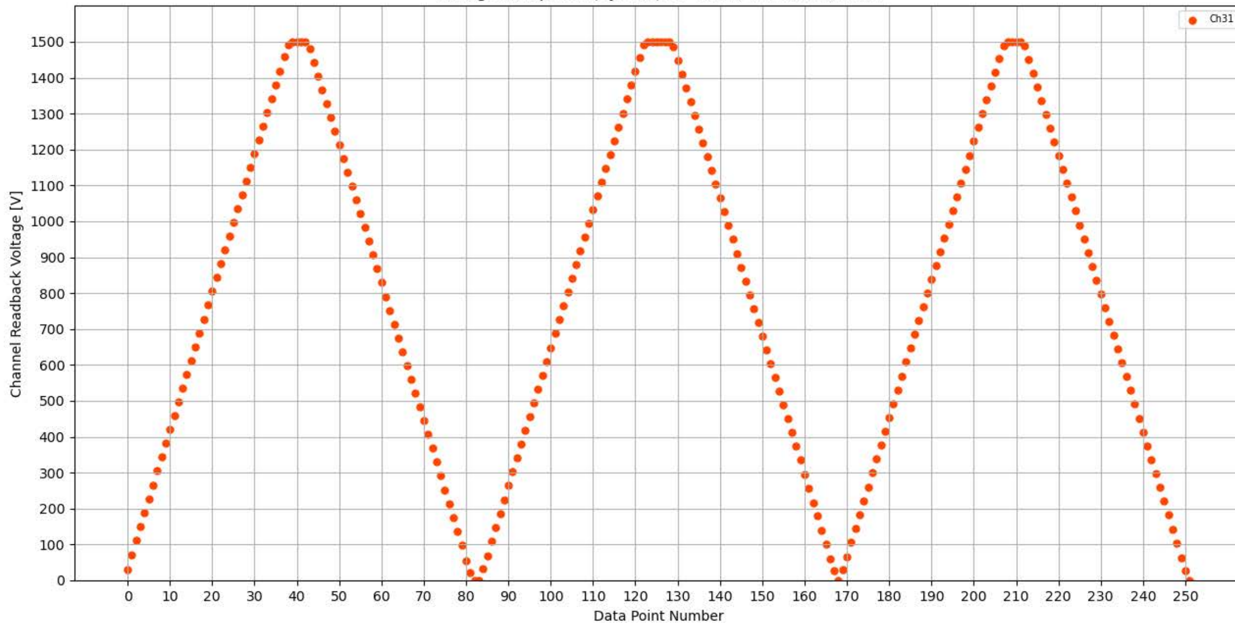
Voltage Ramp Test (Python) Bd #351, Slot #7, Ch #31
