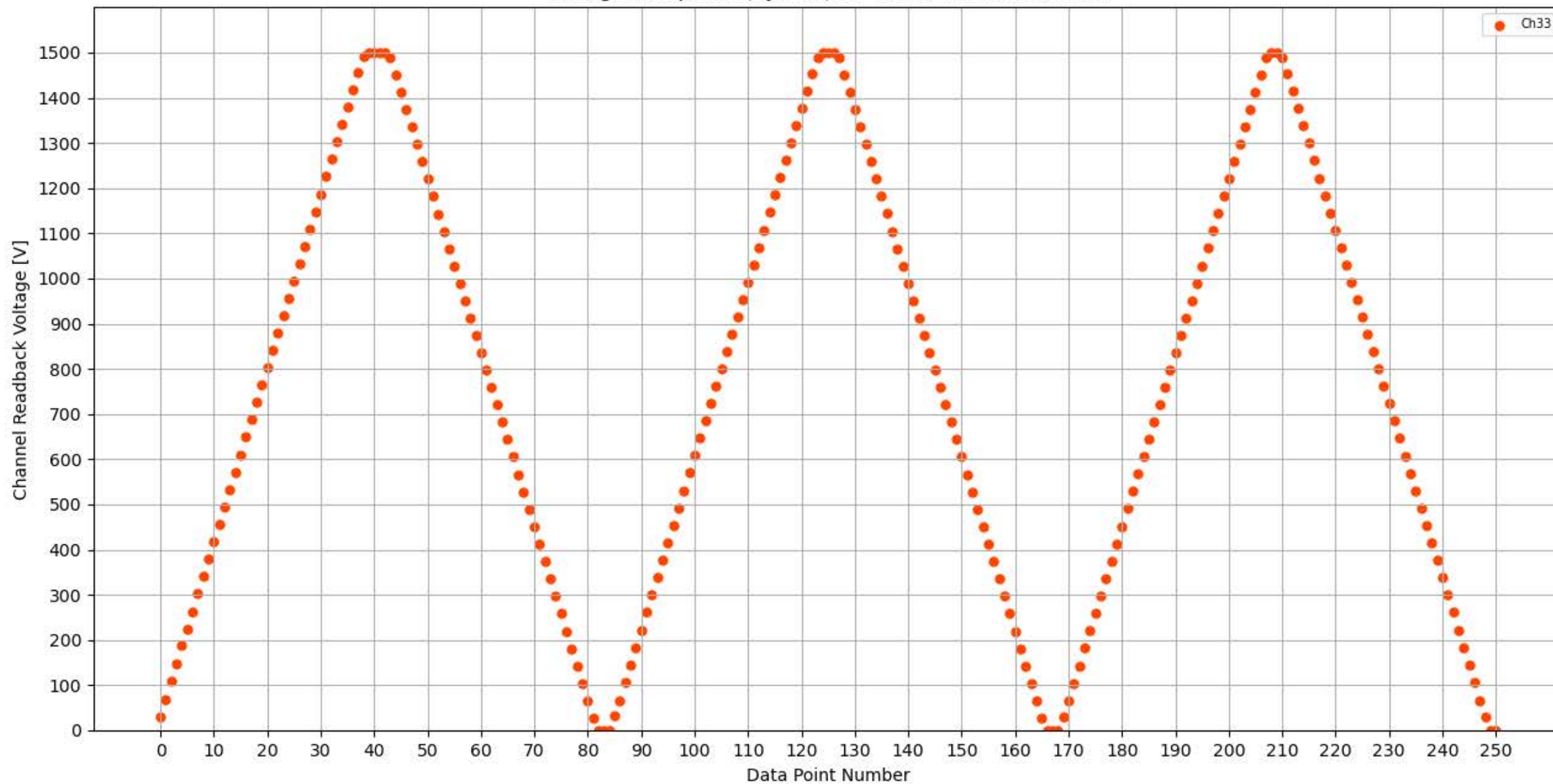
Voltage Ramp Test (Python) Bd #351, Slot #7, Ch #33
