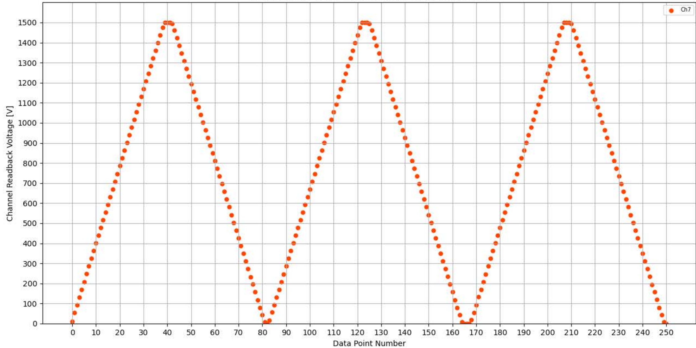
Voltage Ramp Test (Python) Bd #351, Slot #7, Ch #7
