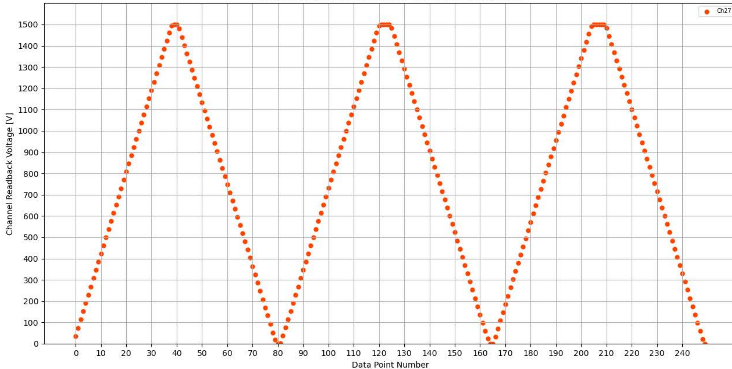
Voltage Ramp Test (Python) Bd #351, Slot #7, Ch #27
