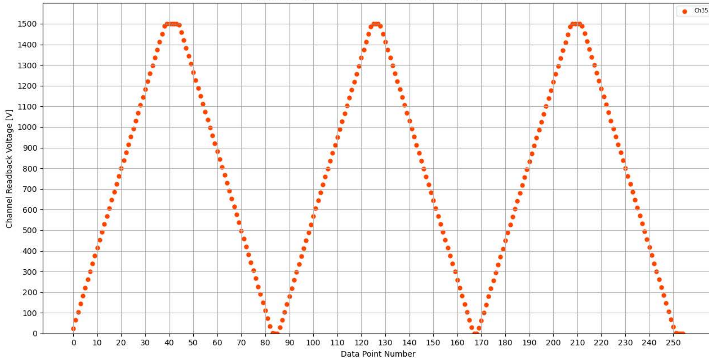
Voltage Ramp Test (Python) Bd #351, Slot #7, Ch #35
