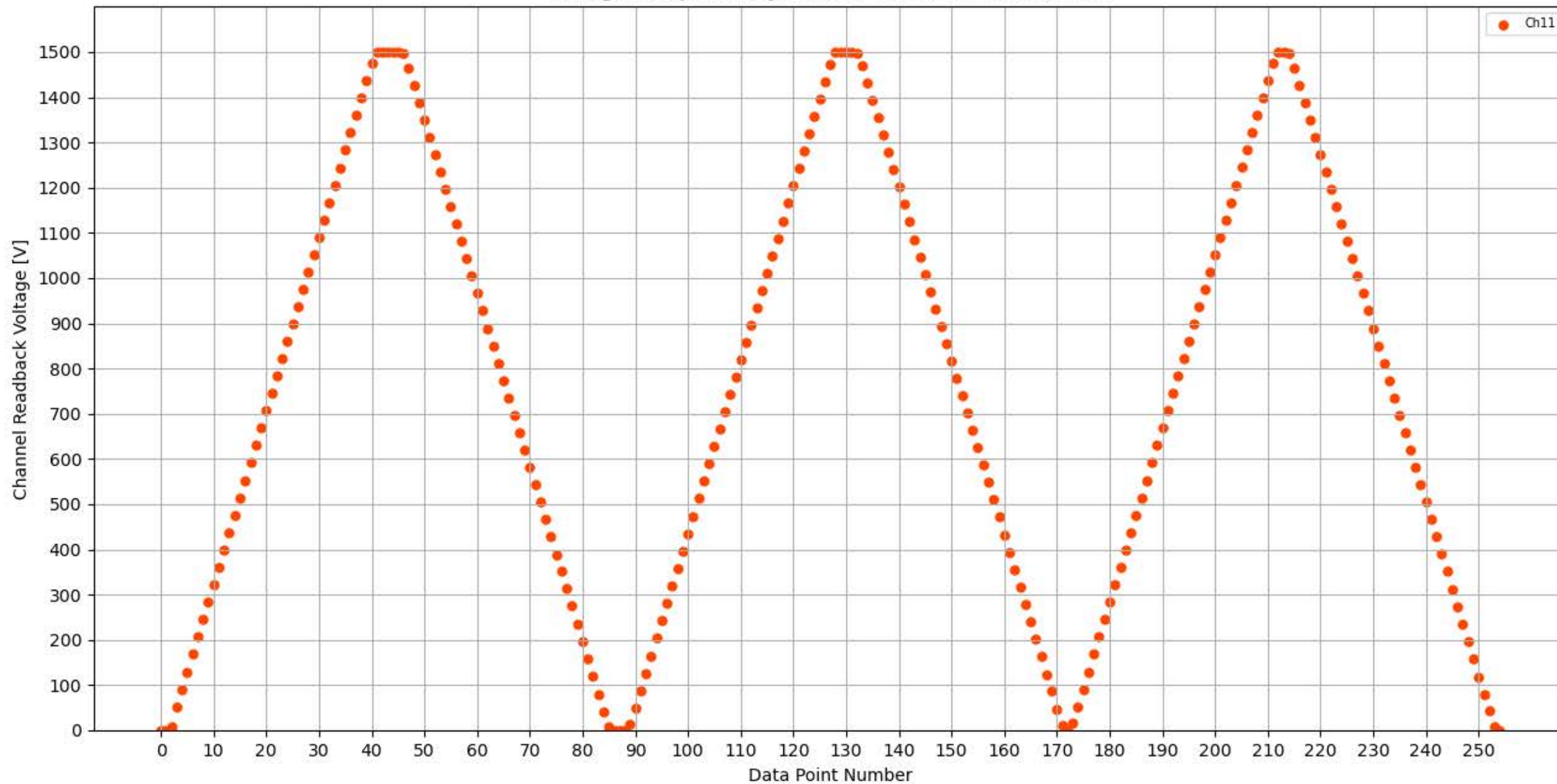
Voltage Ramp Test (Python) Bd #351, Slot #7, Ch #11
