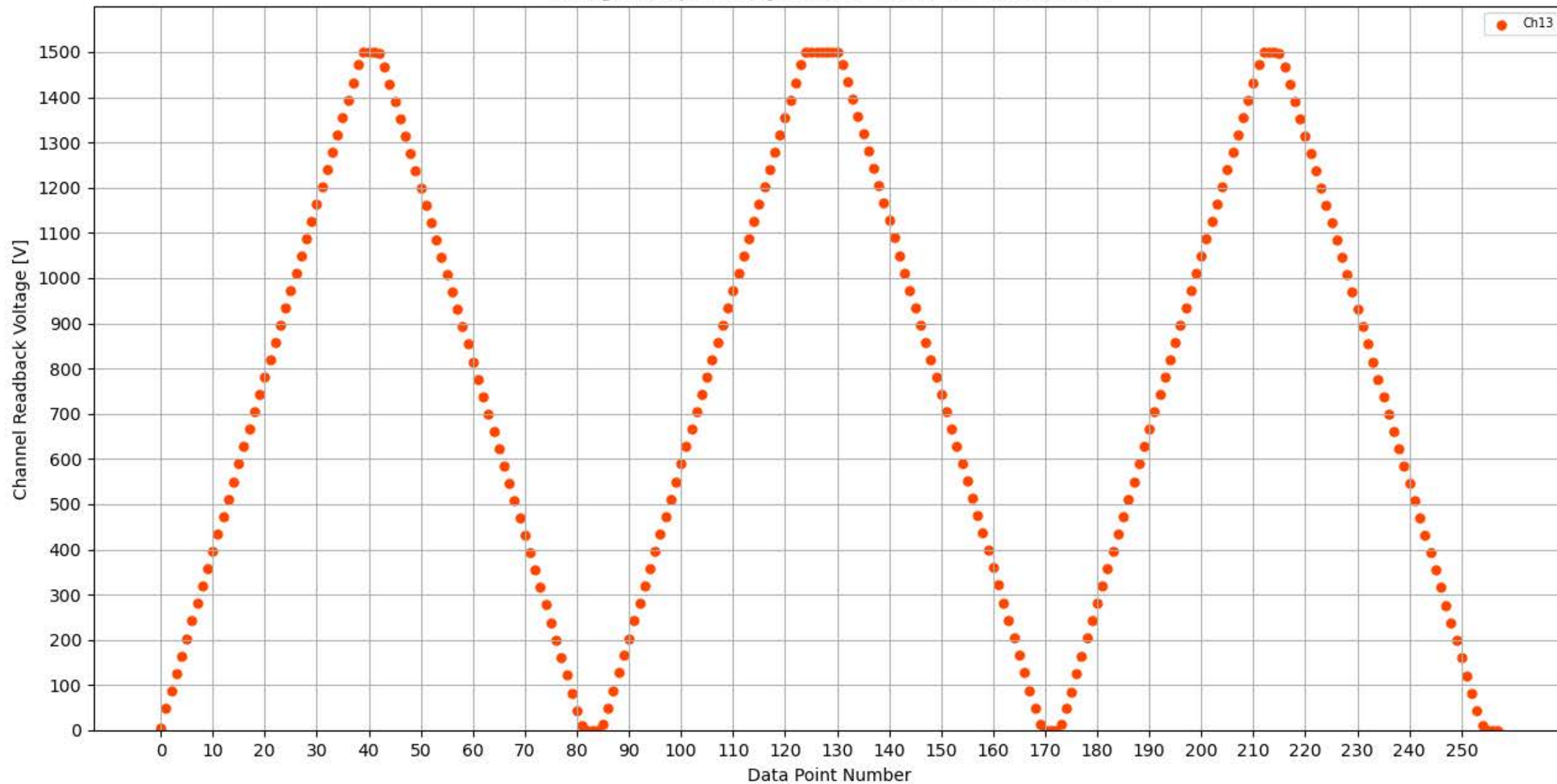
Voltage Ramp Test (Python) Bd #351, Slot #7, Ch #13
