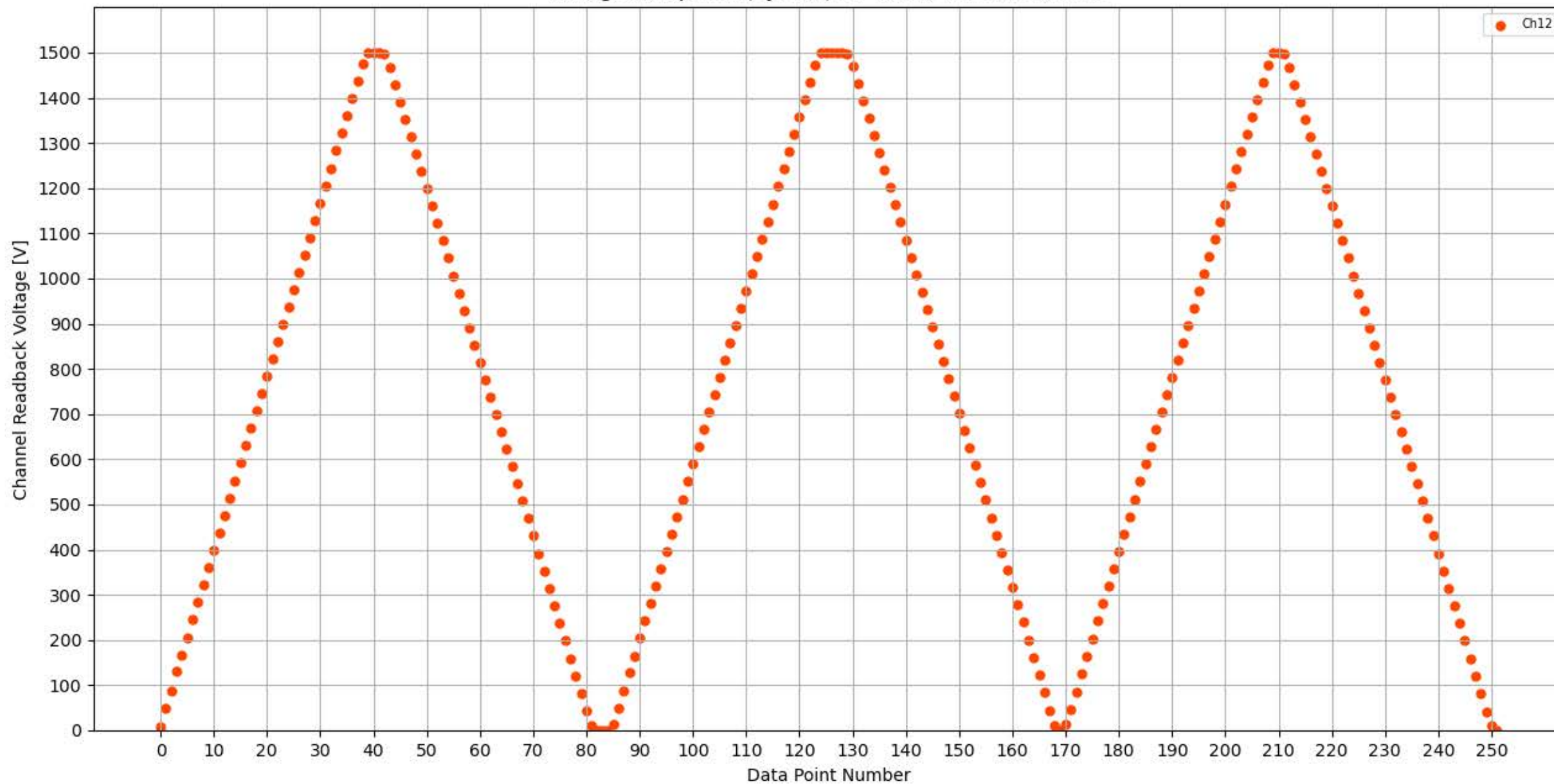
Voltage Ramp Test (Python) Bd #351, Slot #7, Ch #12
