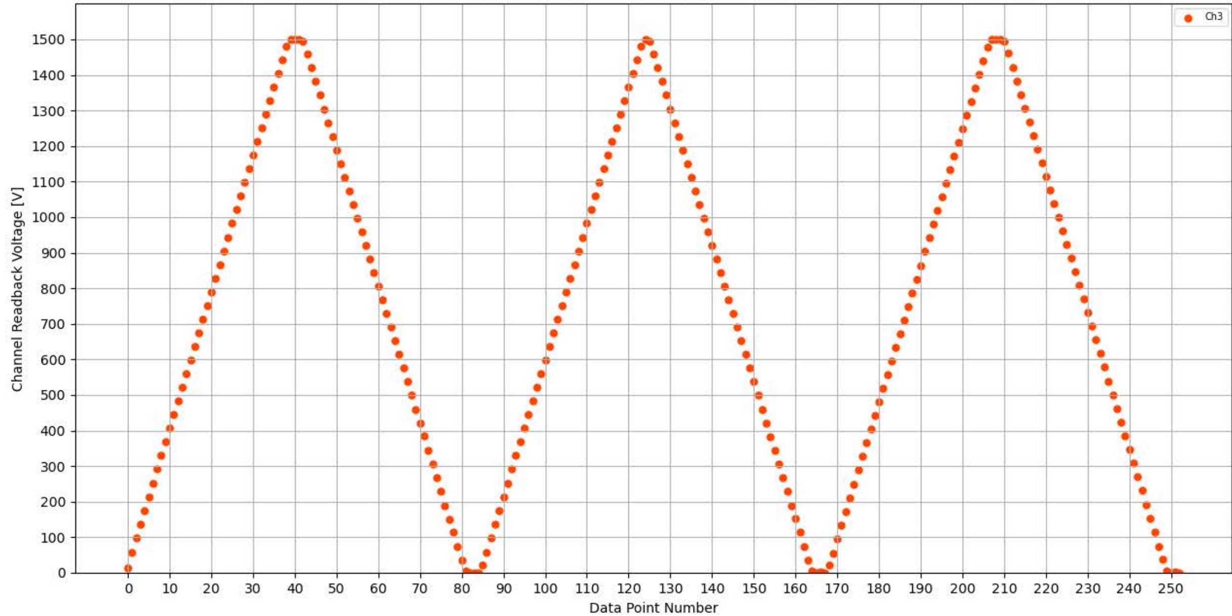
Voltage Ramp Test (Python) Bd #351, Slot #7, Ch #3
