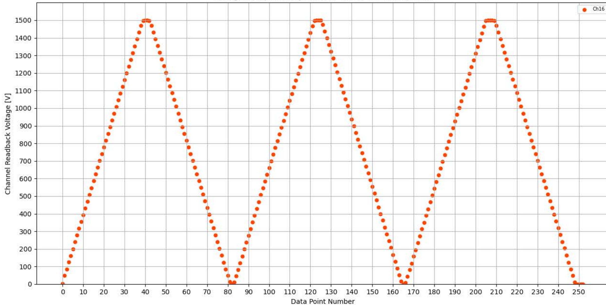
Voltage Ramp Test (Python) Bd #351, Slot #7, Ch #16
