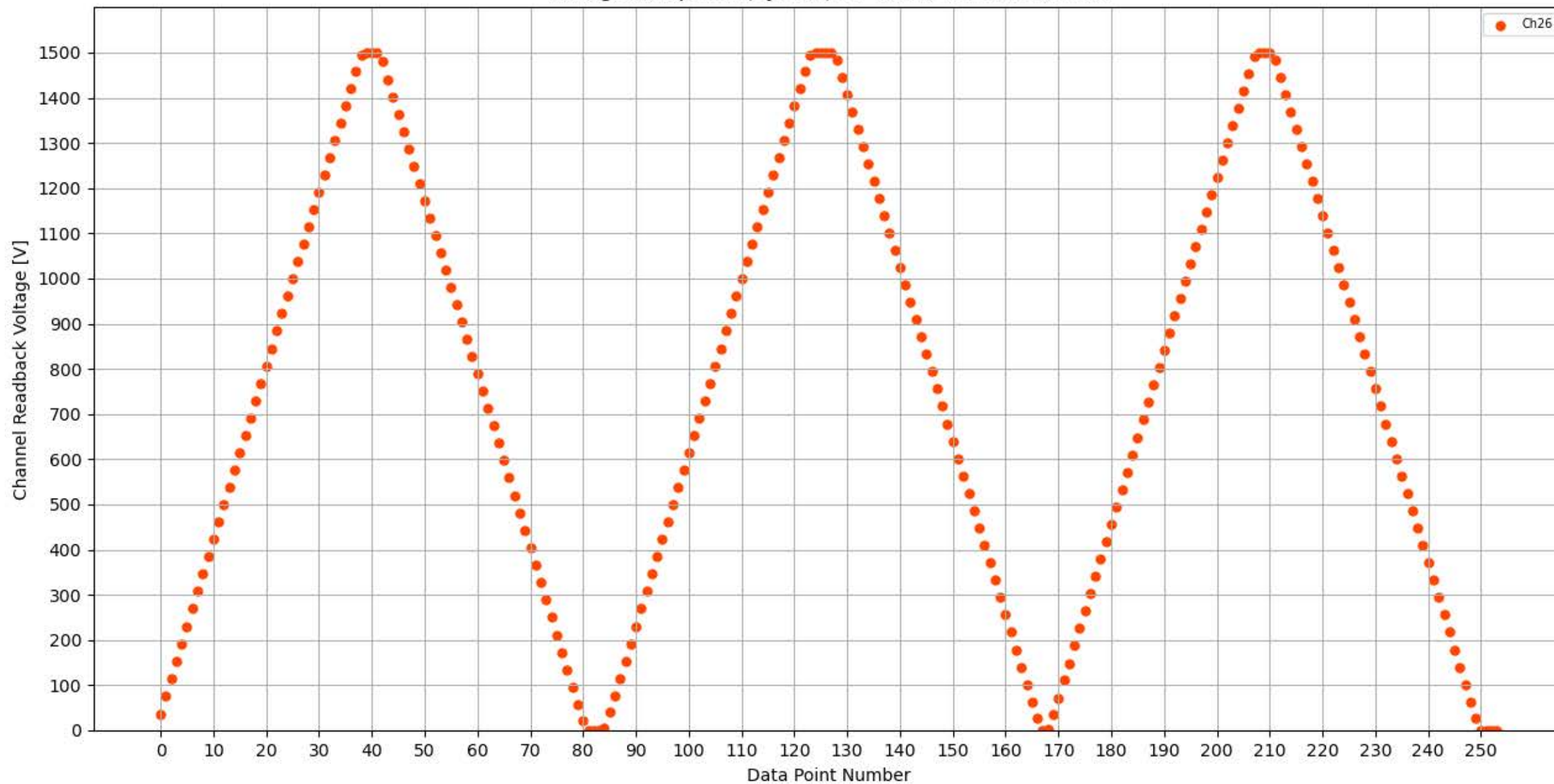
Voltage Ramp Test (Python) Bd #351, Slot #7, Ch #26
