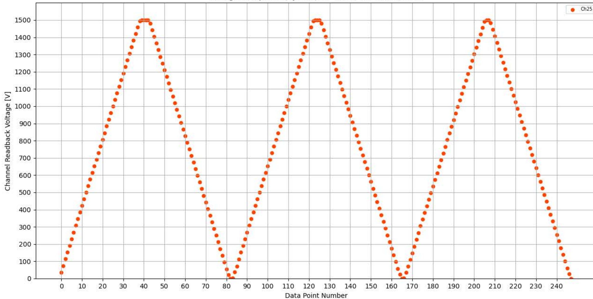
Voltage Ramp Test (Python) Bd #351, Slot #7, Ch #25
