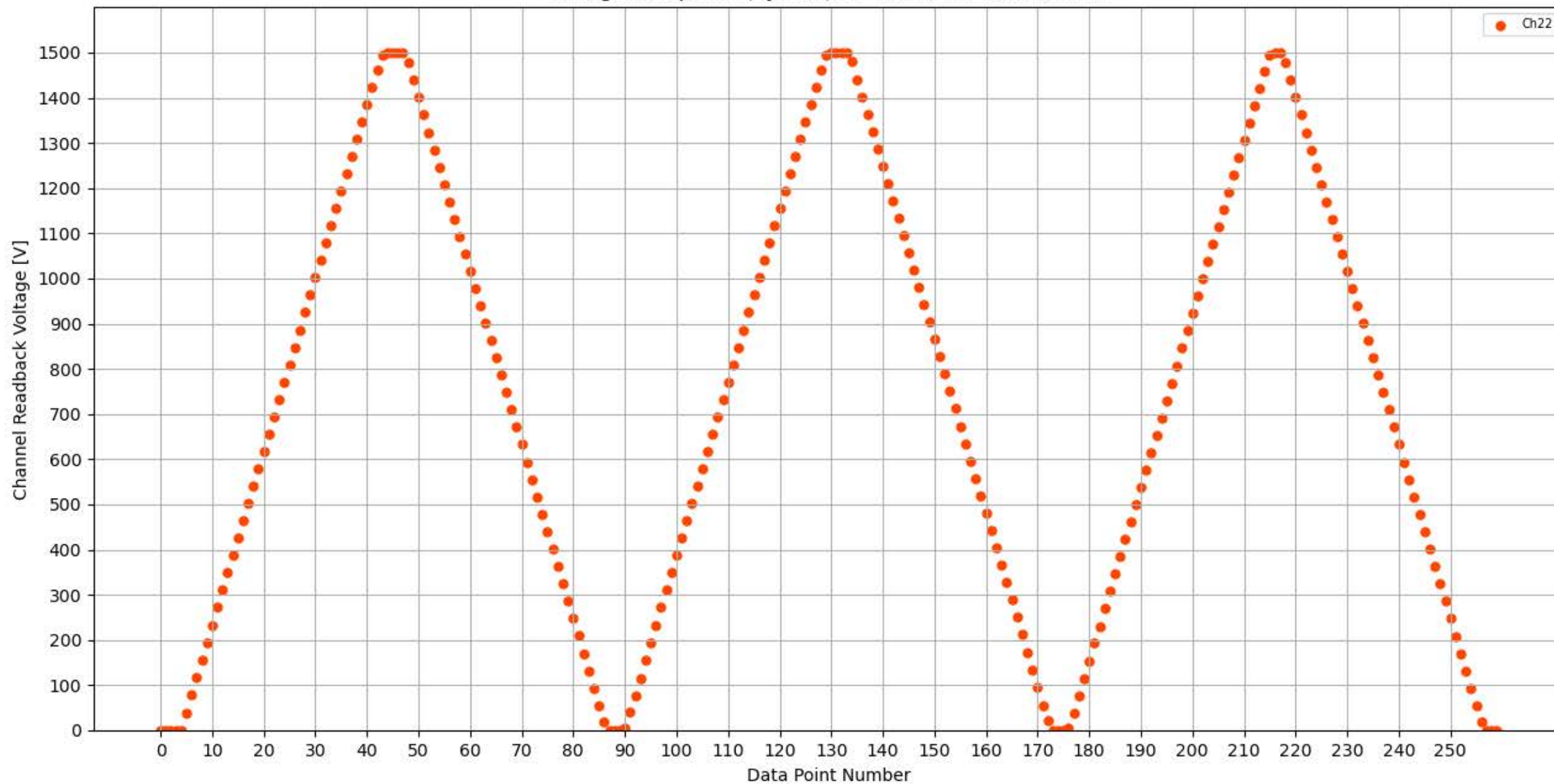
Voltage Ramp Test (Python) Bd #351, Slot #7, Ch #22
