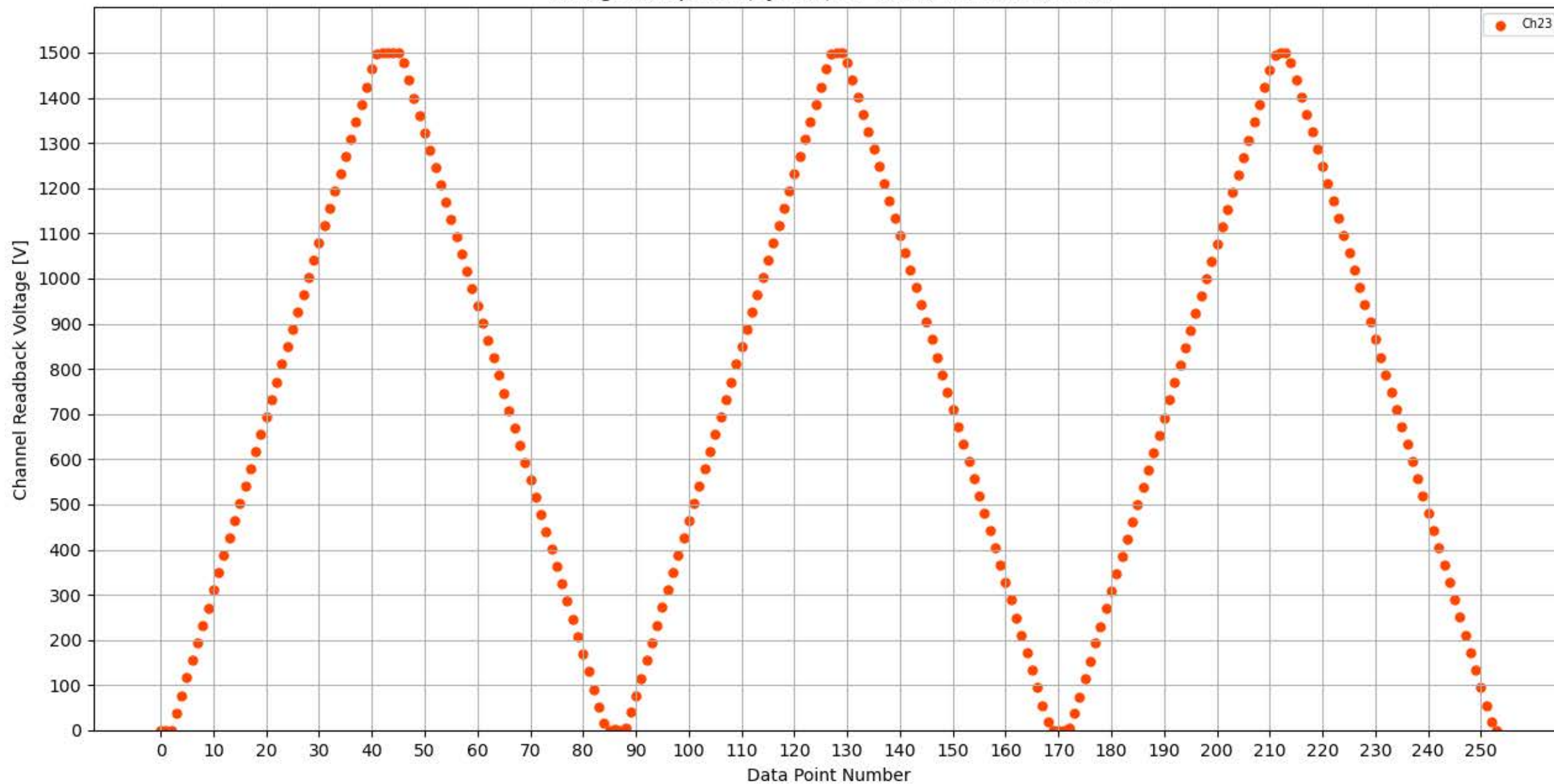
Voltage Ramp Test (Python) Bd #351, Slot #7, Ch #23
