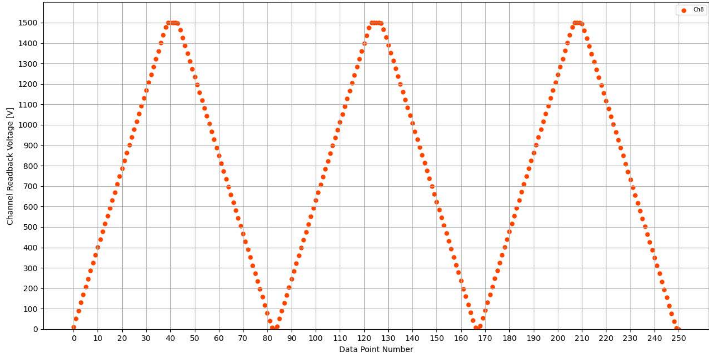
Voltage Ramp Test (Python) Bd #351, Slot #7, Ch #8
