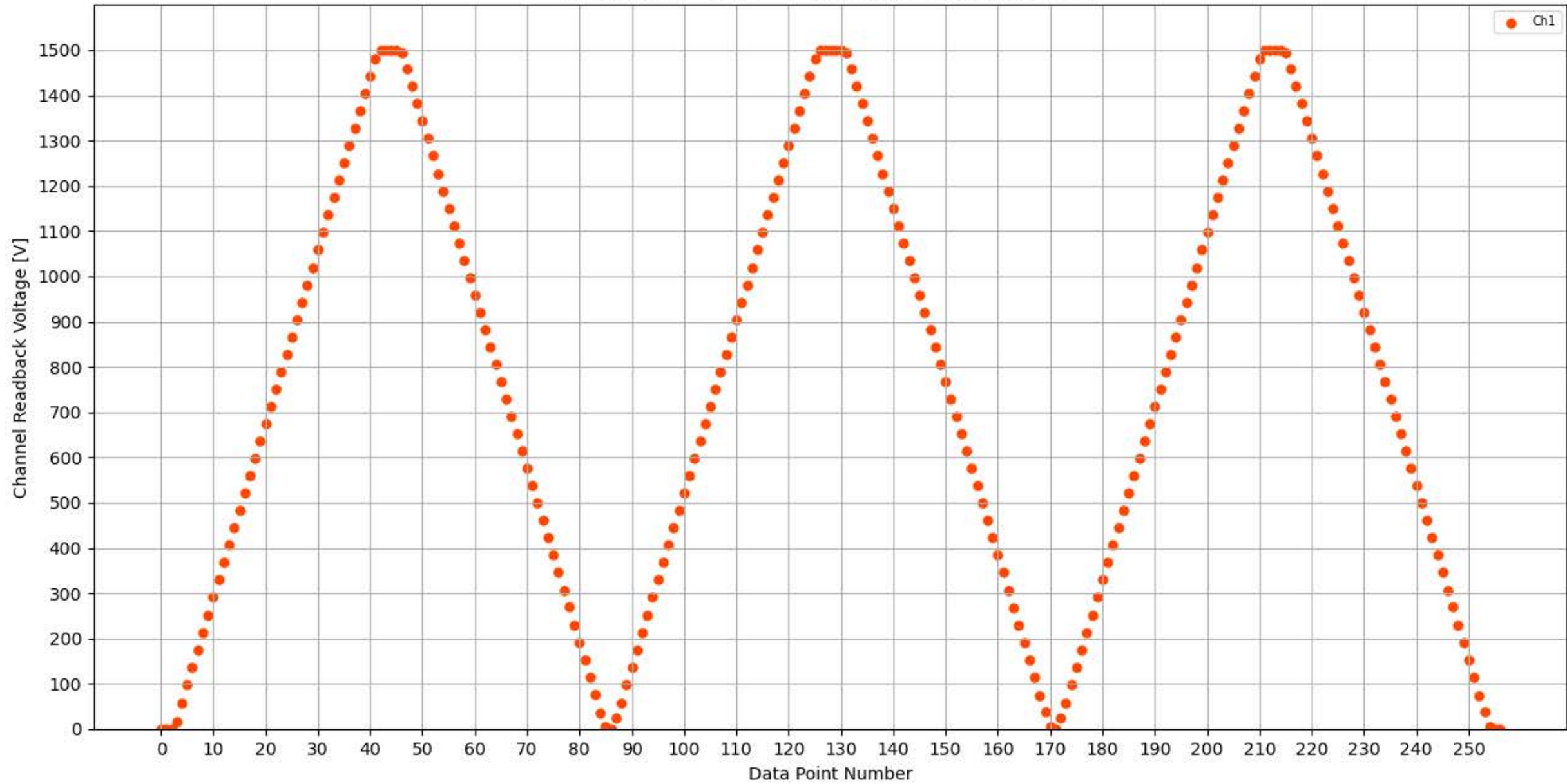
Voltage Ramp Test (Python) Bd #351, Slot #7, Ch #1
