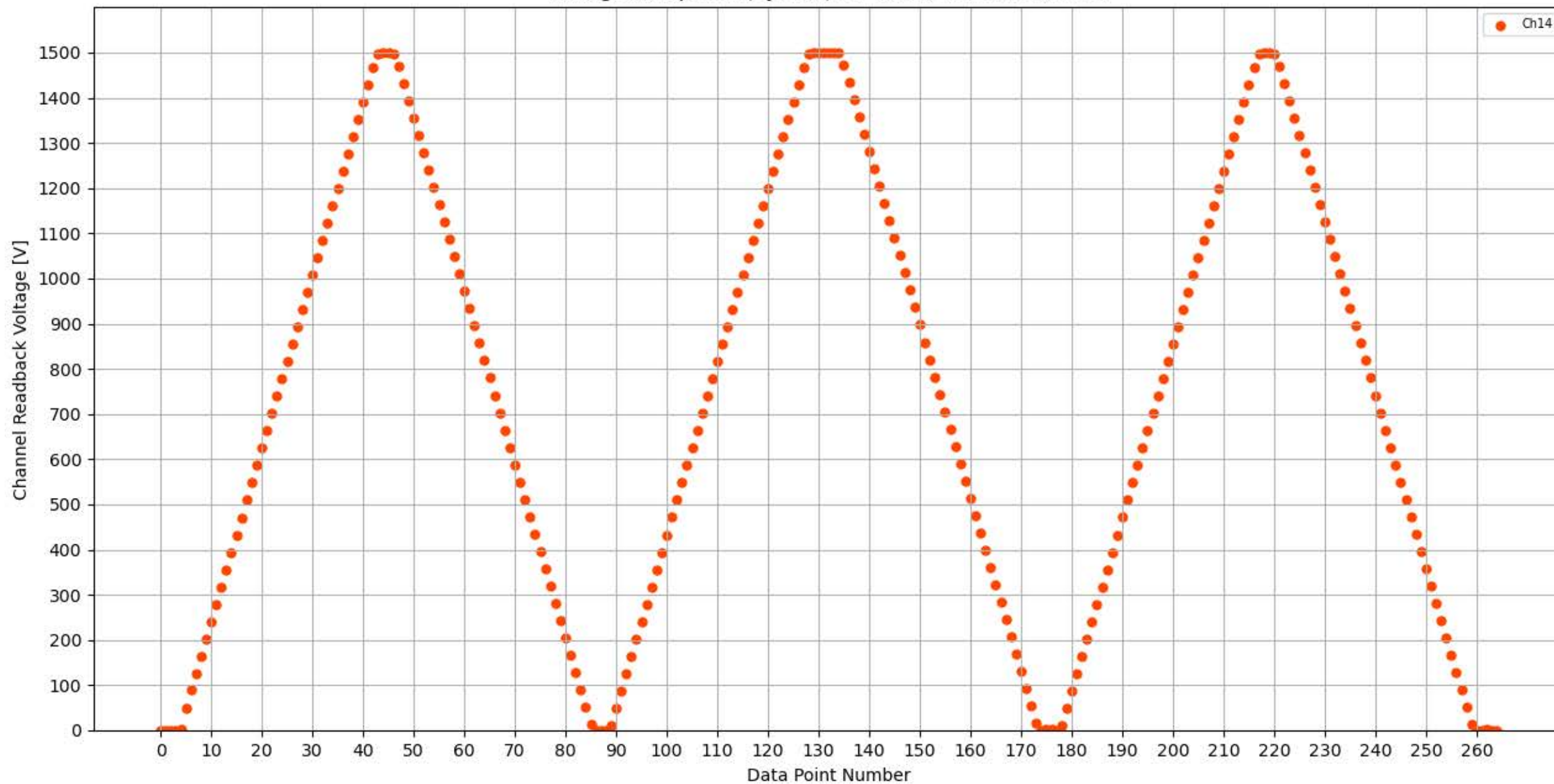
Voltage Ramp Test (Python) Bd #351, Slot #7, Ch #14
