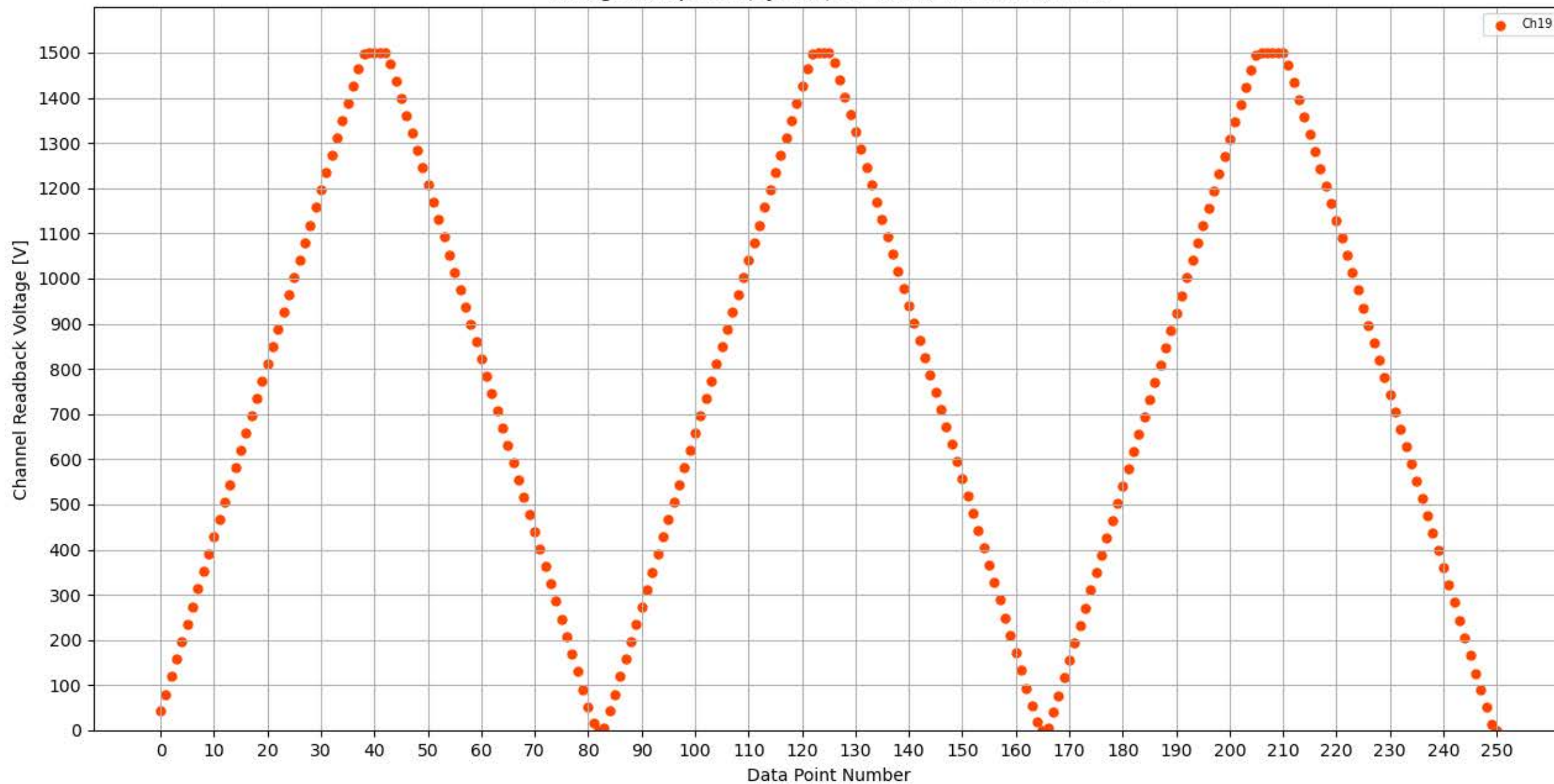
Voltage Ramp Test (Python) Bd #351, Slot #7, Ch #19
