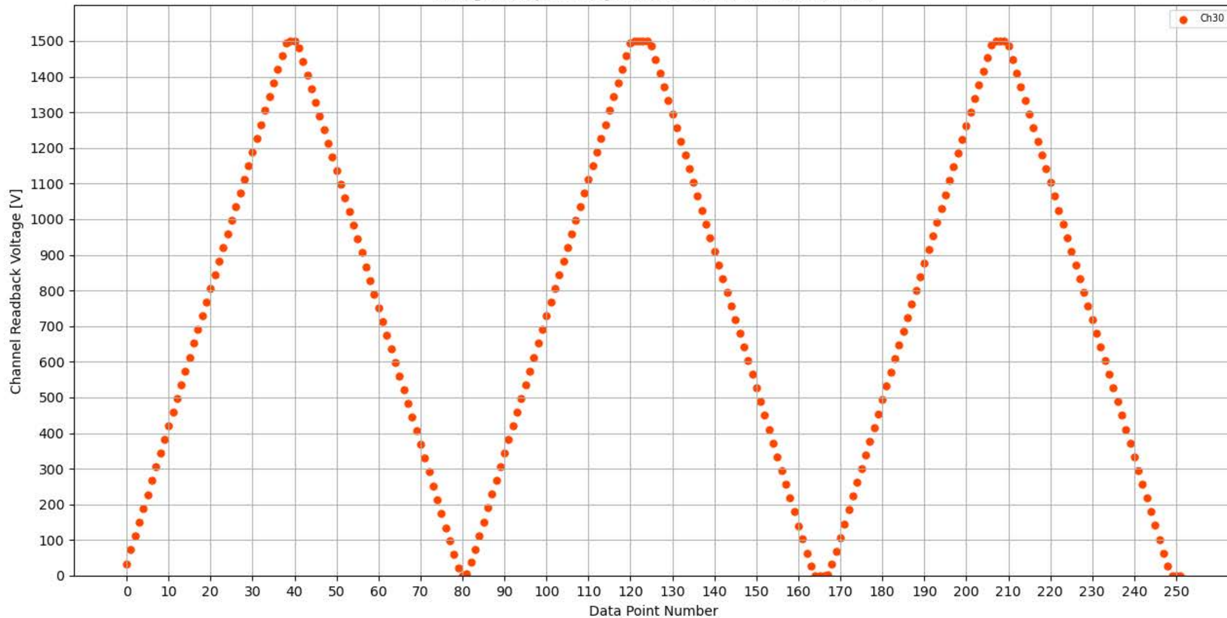
Voltage Ramp Test (Python) Bd #351, Slot #7, Ch #30
