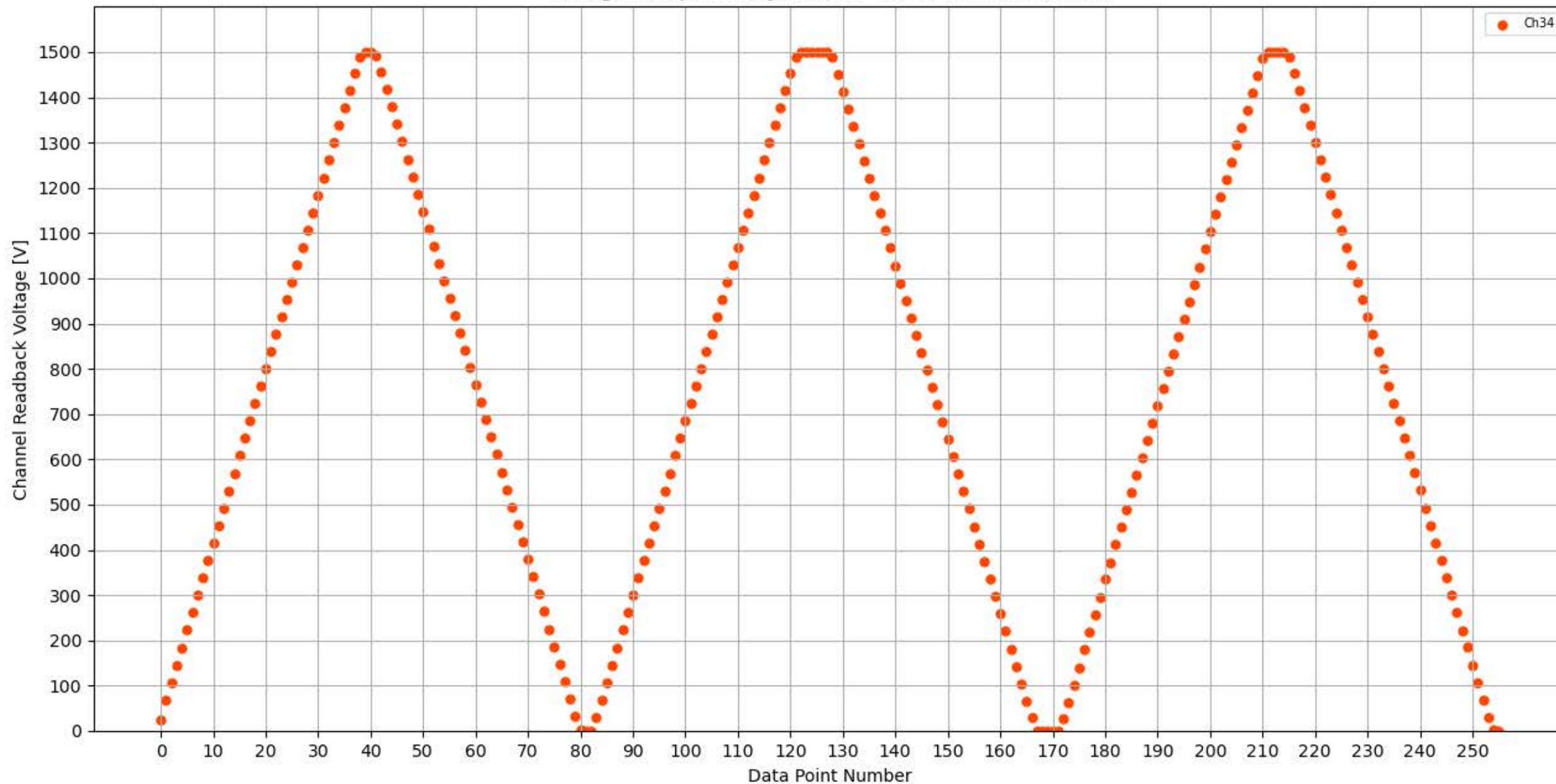
Voltage Ramp Test (Python) Bd #351, Slot #7, Ch #34
