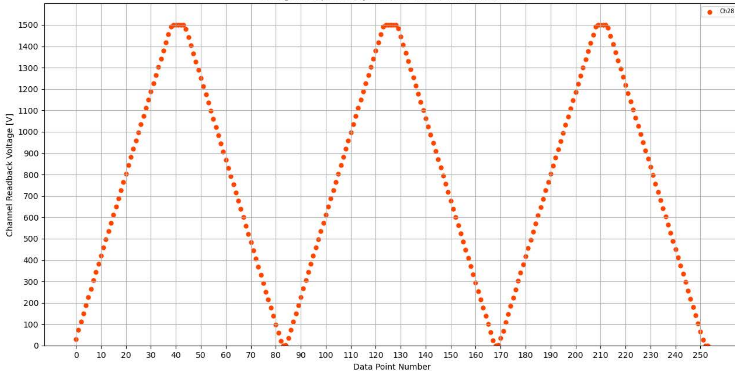
Voltage Ramp Test (Python) Bd #351, Slot #7, Ch #28
