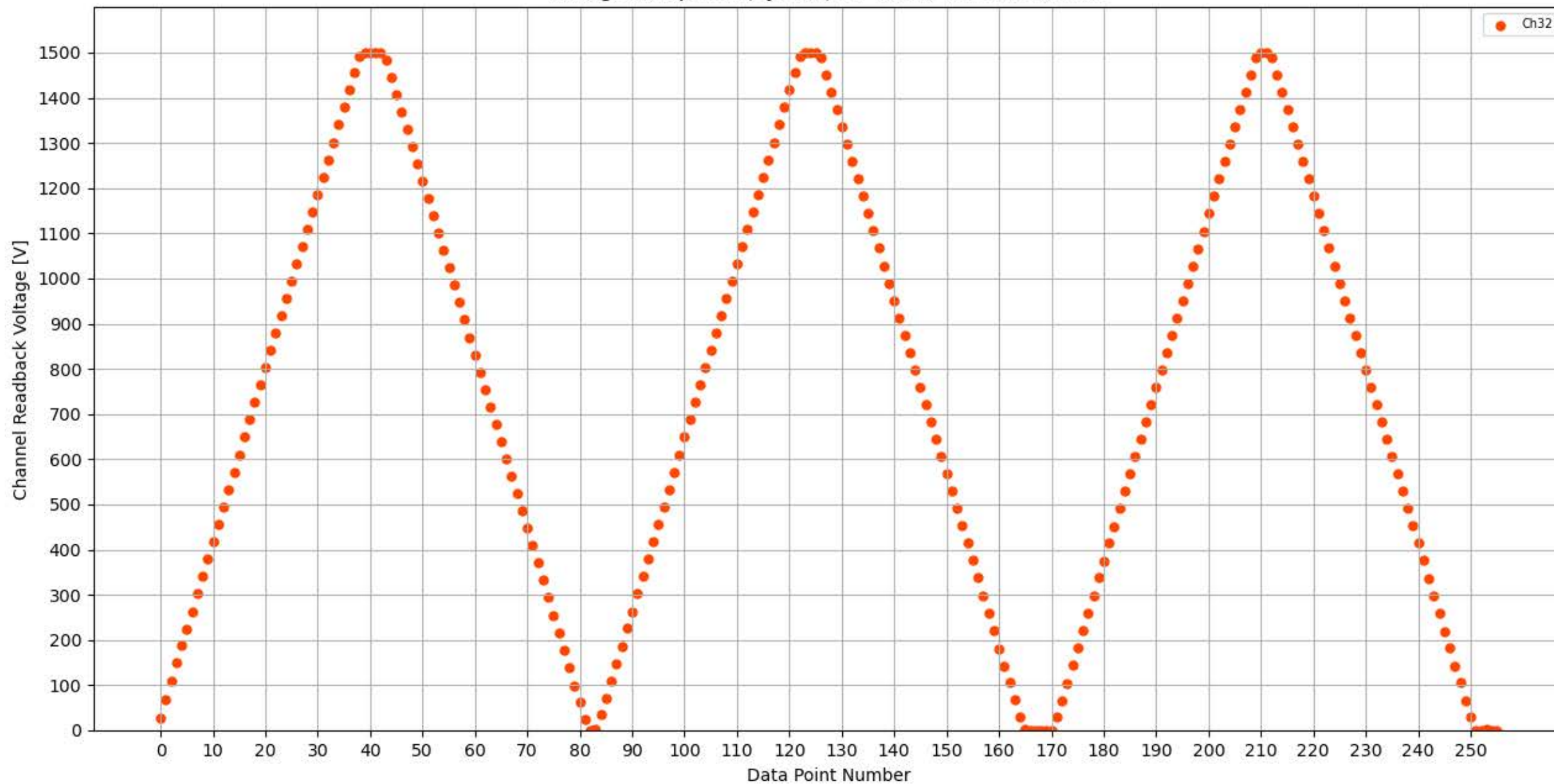
Voltage Ramp Test (Python) Bd #351, Slot #7, Ch #32
