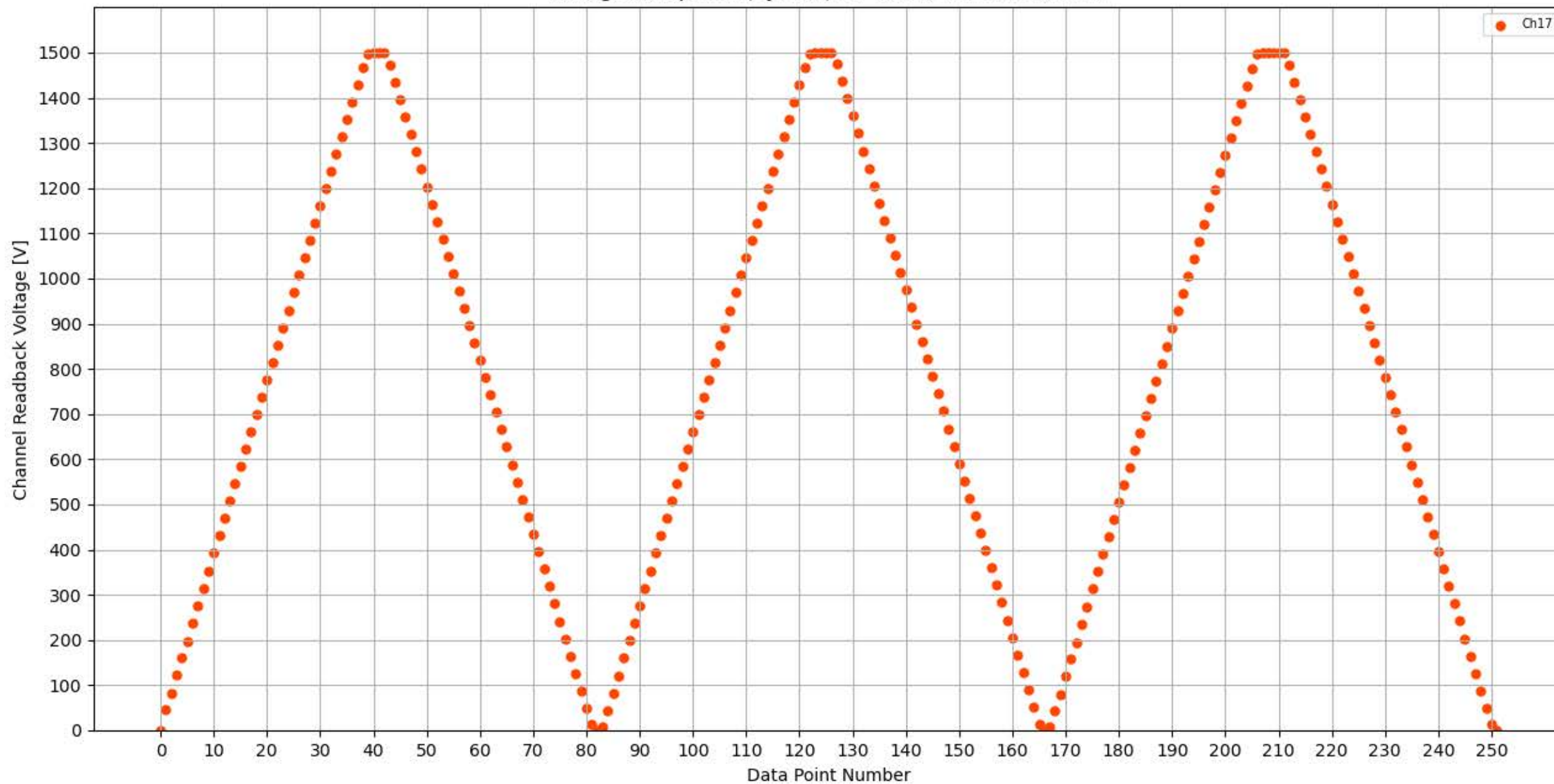
Voltage Ramp Test (Python) Bd #351, Slot #7, Ch #17
