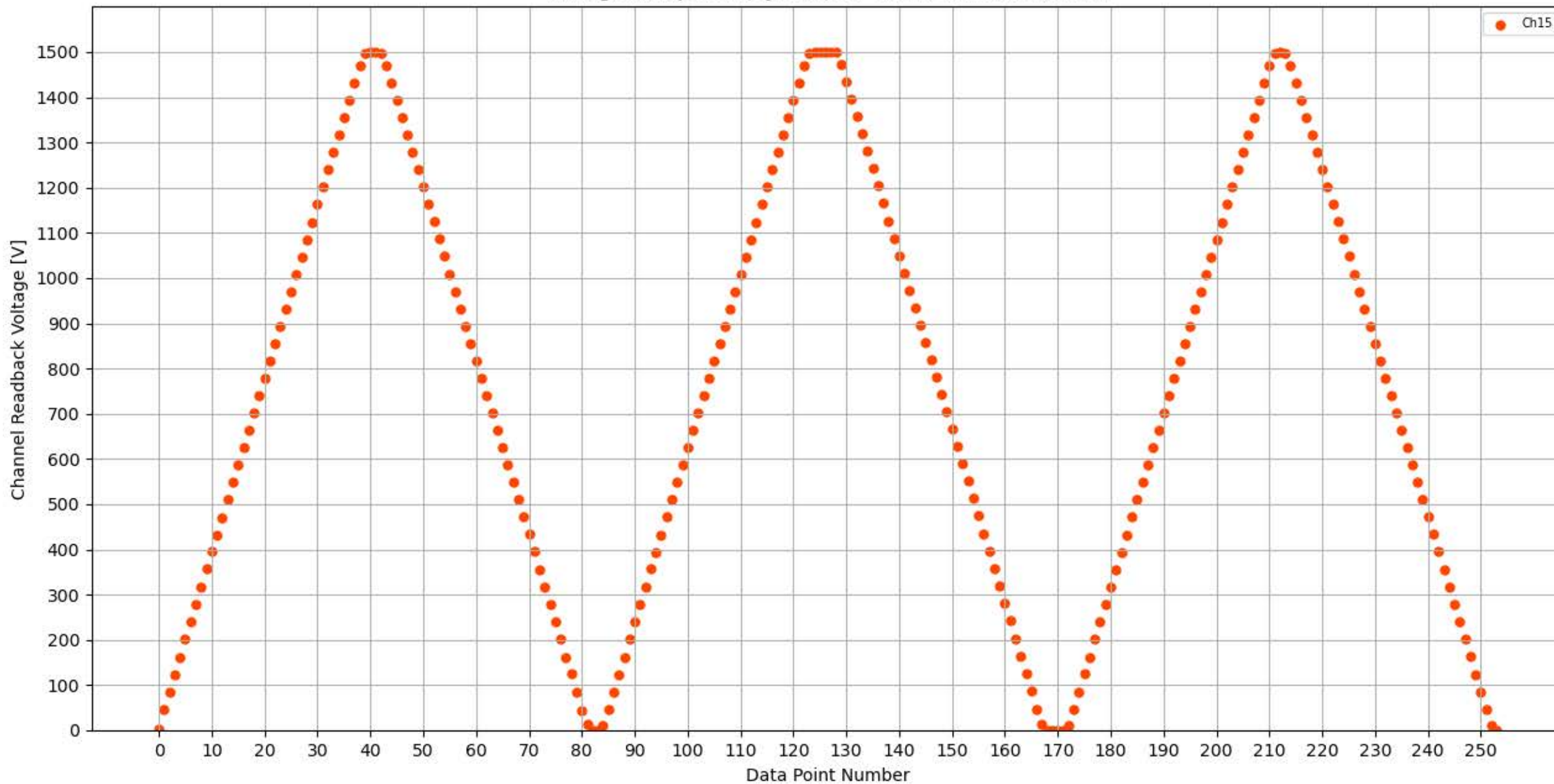
Voltage Ramp Test (Python) Bd #351, Slot #7, Ch #15
