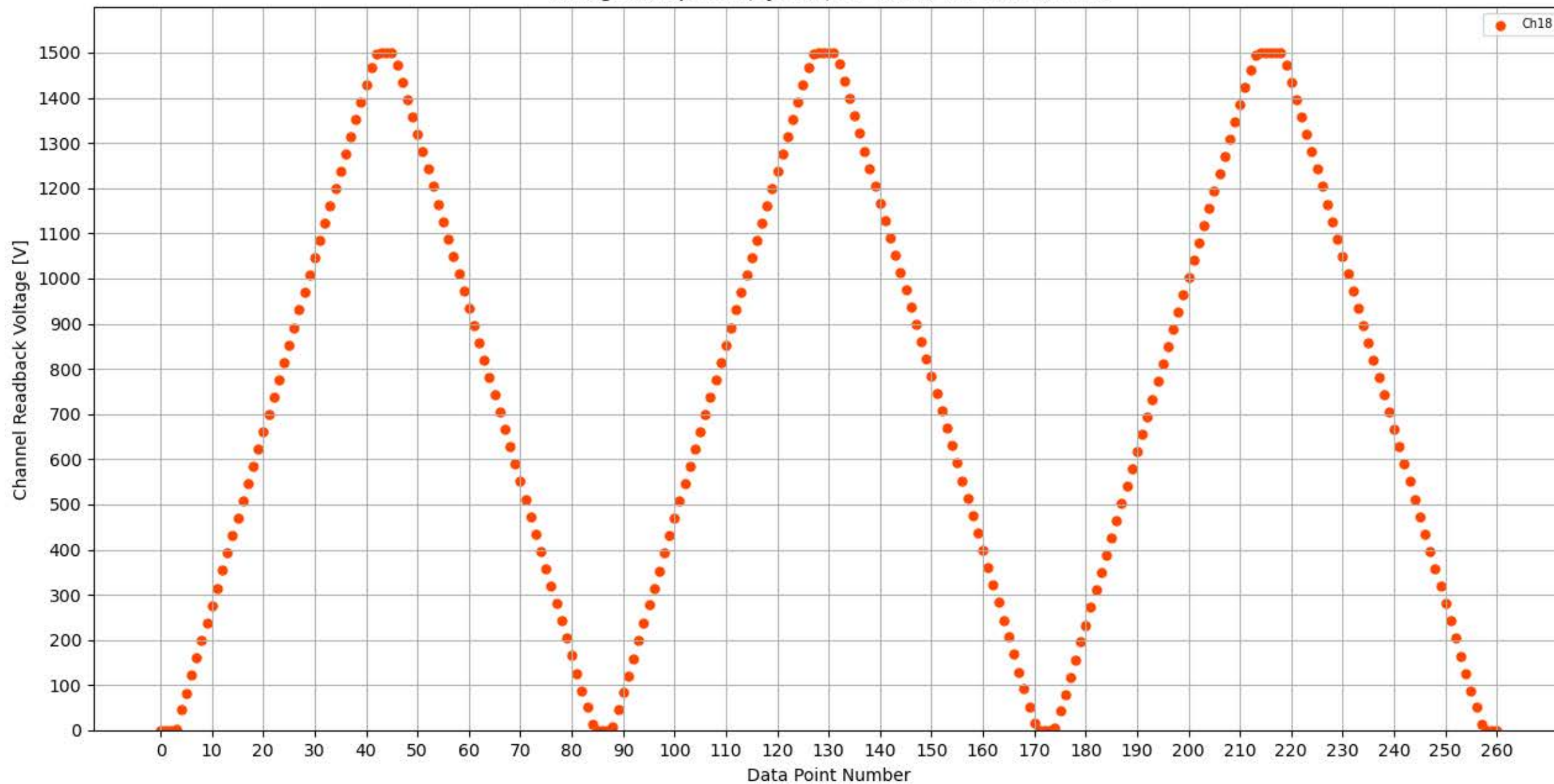
Voltage Ramp Test (Python) Bd #351, Slot #7, Ch #18
