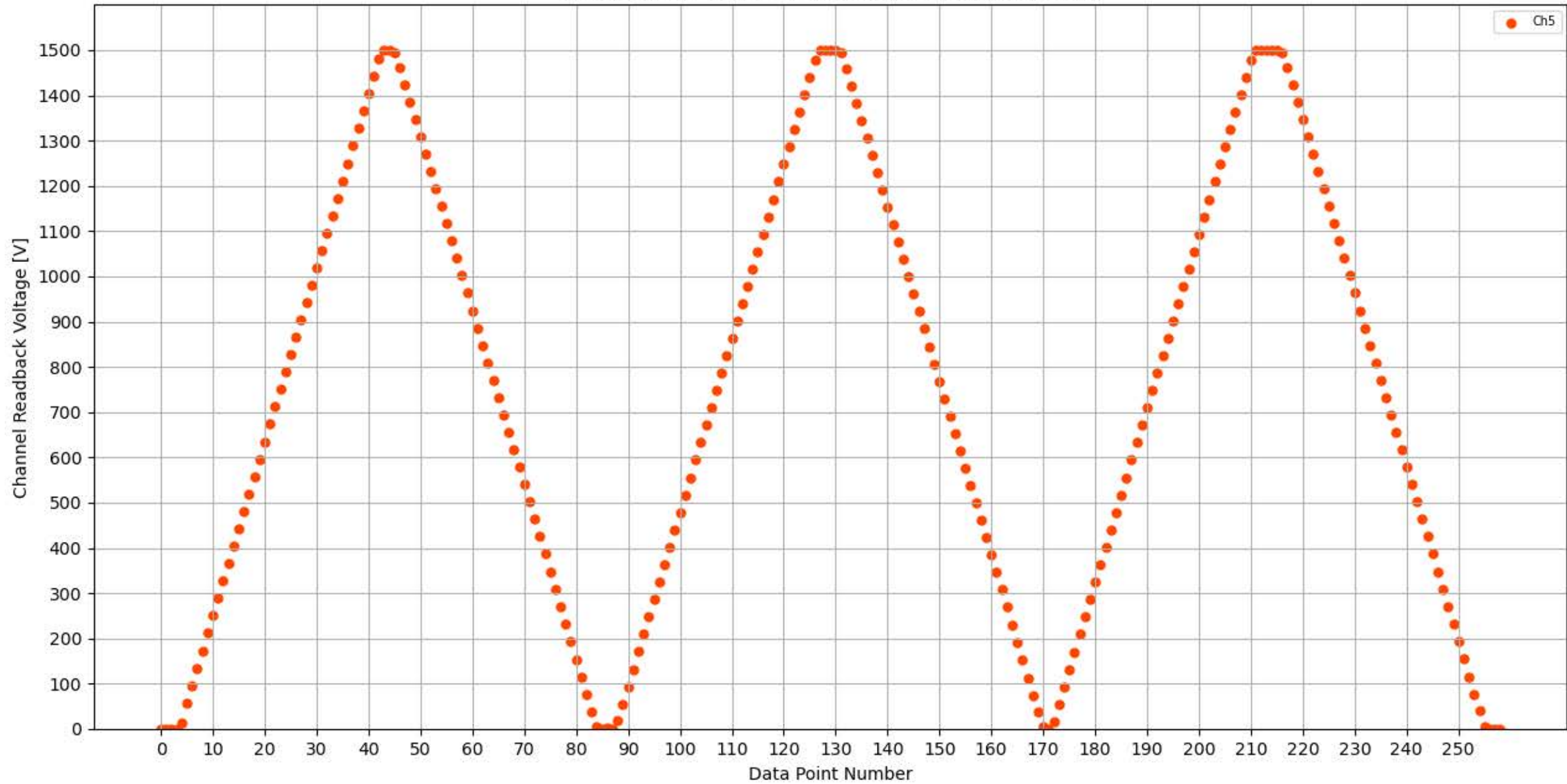
Voltage Ramp Test (Python) Bd #351, Slot #7, Ch #5
