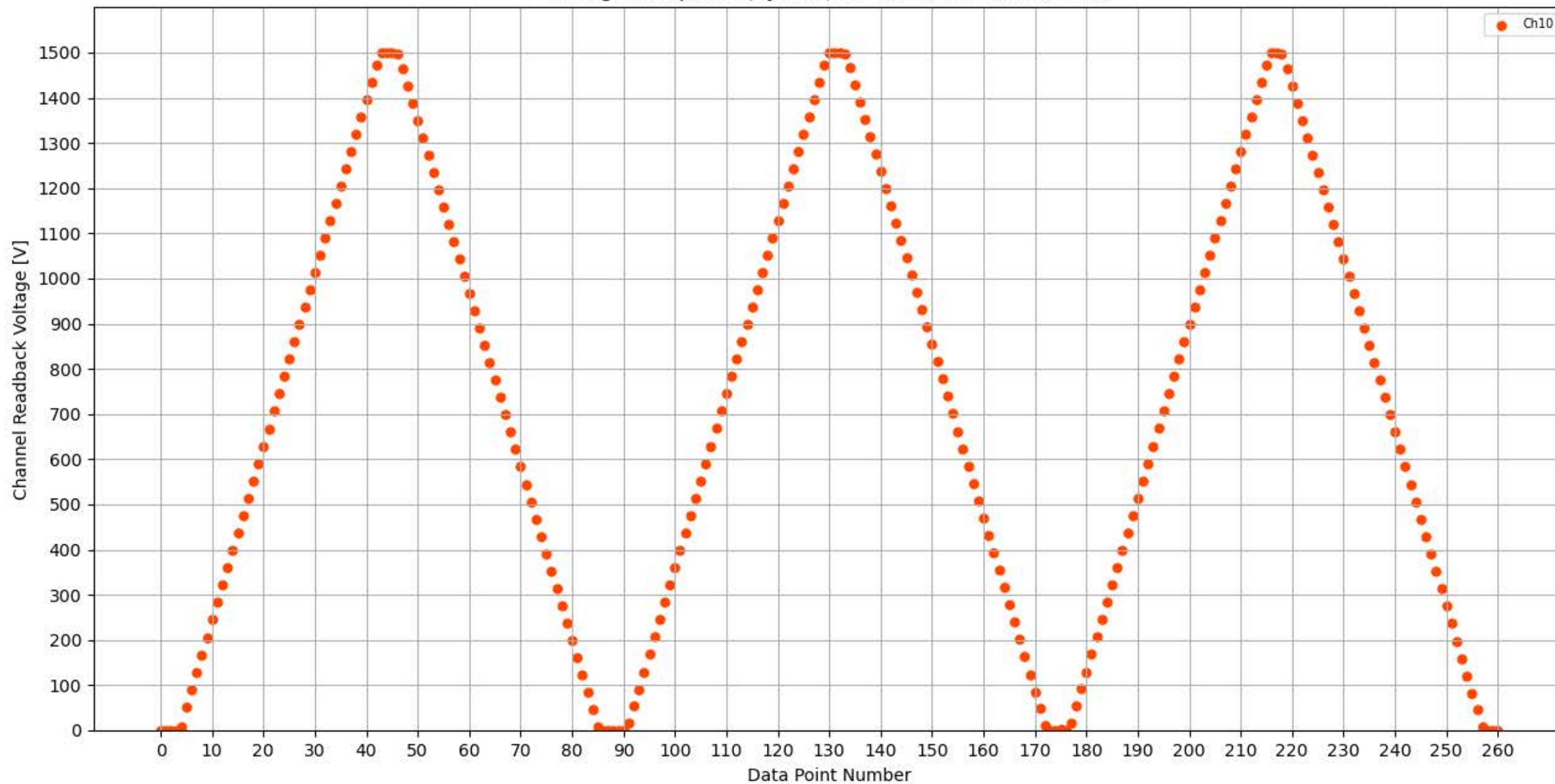
Voltage Ramp Test (Python) Bd #351, Slot #7, Ch #10
