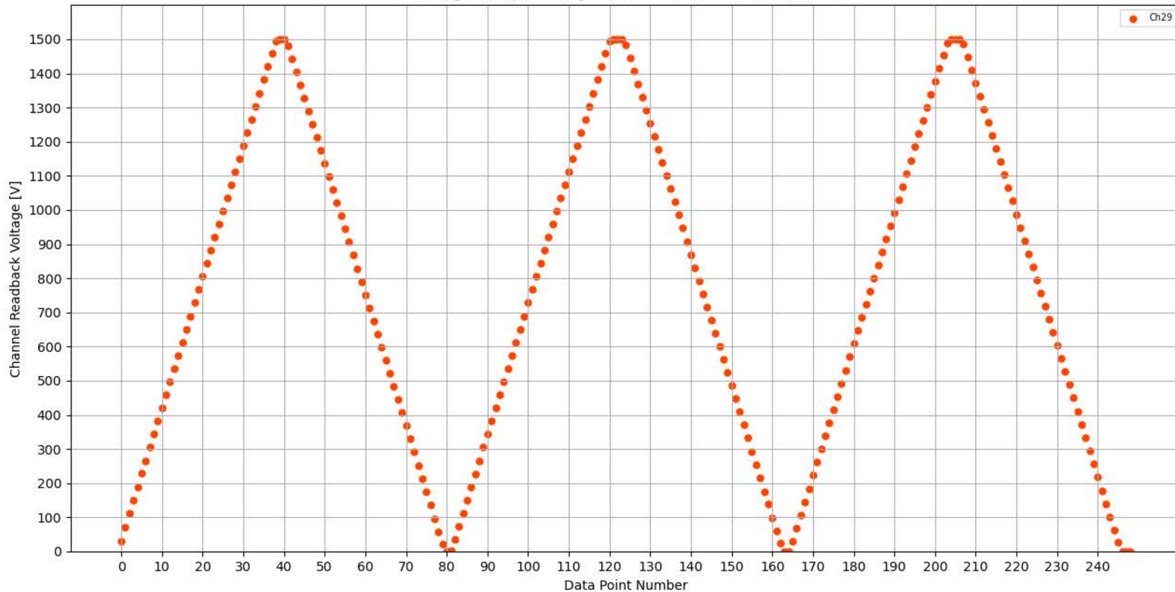
Voltage Ramp Test (Python) Bd #351, Slot #7, Ch #29
